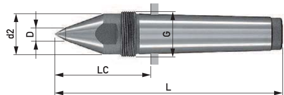
Form 256 Kopierform 60°/40°
